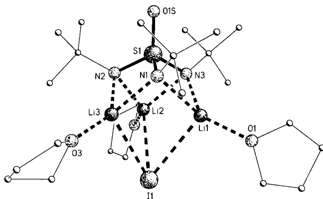
Fig. 5. Solid state structure of [\text{thf}_3\text{Li}_3\{\mu_3\text{-I}(\text{N}^t\text{Bu})_3\text{SO}\}] .
