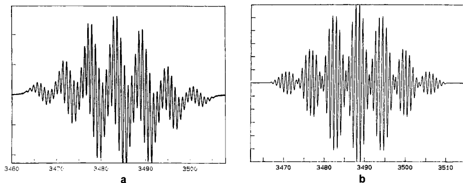
Fig. 4. Experimental ESR-spectrum (a) from oxidized [\text{Li}_4\{(\text{N}^t\text{Bu})_3\text{S}\}_2] in hexane solution in comparison to the calculated spectrum of [\text{Li}\{(\text{N}^t\text{Bu})_3\text{S}\}_2]^\bullet (b).
