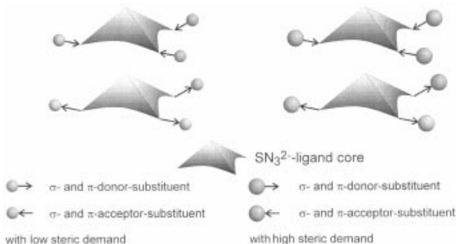
Fig. 10. Electronic and steric fine tuning of the \text{S}(\text{NR})_3 cap.
