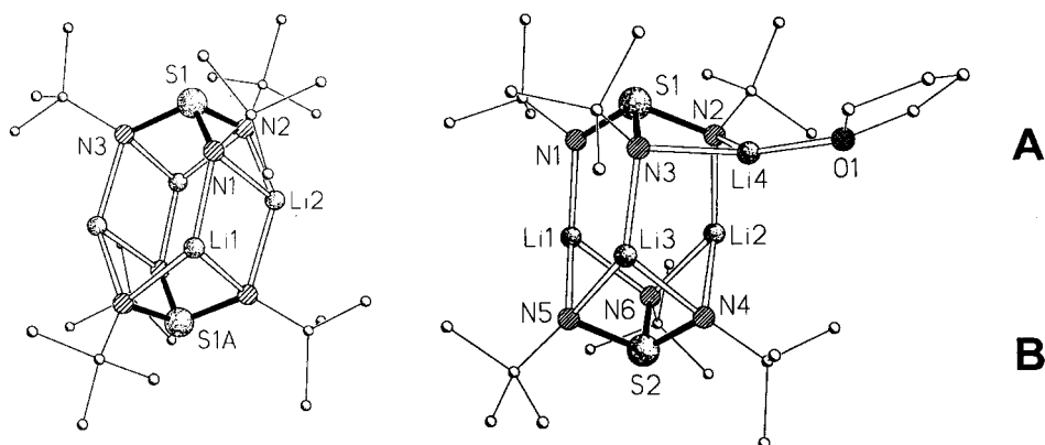
Fig. 3. Solid state structures of [\text{Li}(\text{N}^t\text{Bu})_3\text{S}]_2 and [(\text{thf})\text{Li}_4\{(\text{N}^t\text{Bu})_3\text{S}\}_2] .
